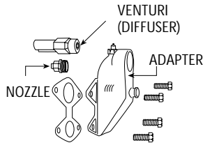
Shallow Well Package
